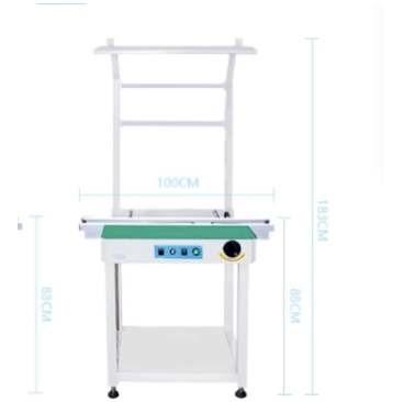
TOKii-1000IC / TOKii-IC600 TOKii® INLINE INSPECTION CONVEYOR
