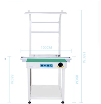
TOKii-1000IC / TOKii-IC600 INLINE INSPECTION CONVEYOR TOKii®
