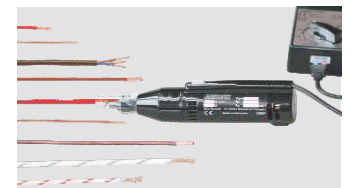
A1LM for 0.2-0.8 mm Diameter A3LM for 0.6-2.0 mm Diameter A5LM for 1.2-4.5 mm Diameter
