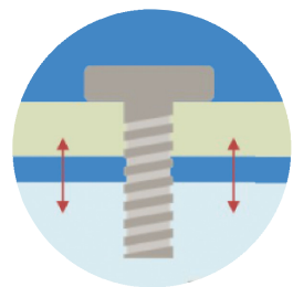
浮牙檢測 Floating screw
